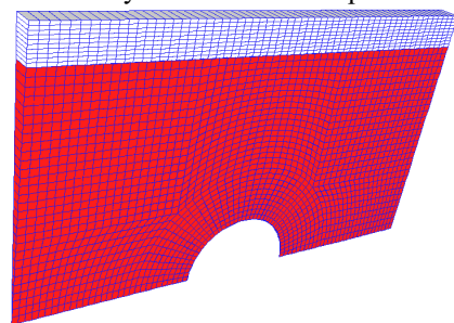
Fig. 2: Wedge mesh topology
