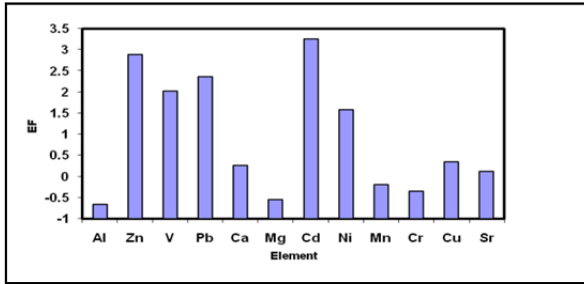
Figure 3. Enrichment of elements in the study area
