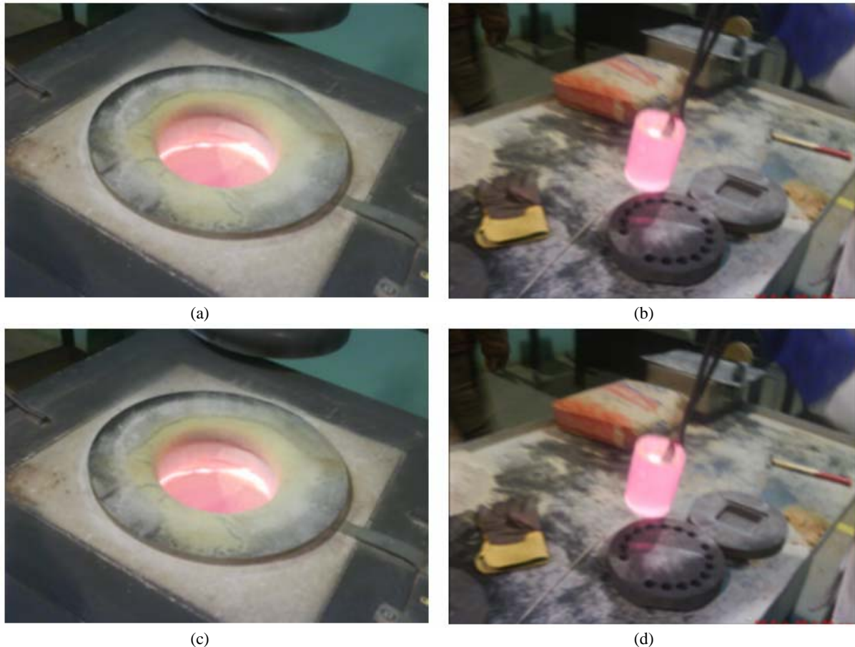
Figure 3 Casting steps: (a) crucible at induction furnace, (b) & (c) pouring, and (d) cast specimens after cooling
