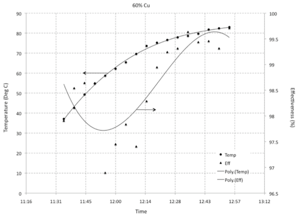
Figure 8 Temperature rise and effectiveness for 60% Cu content
