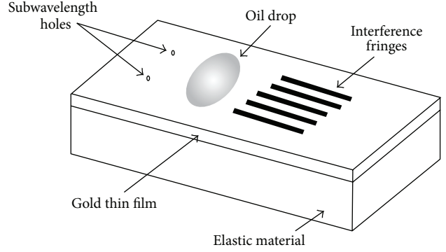
FIGURE 1: Experimental setup to generate the incoherent convergence of Spc. The width of the gold thin film is 40 nm placed on an elastic material. The relative position between holes is in the interval 5–15 nm and it is controlled applying a random force. The refractive index for the oil drop is n = 2.1 .
