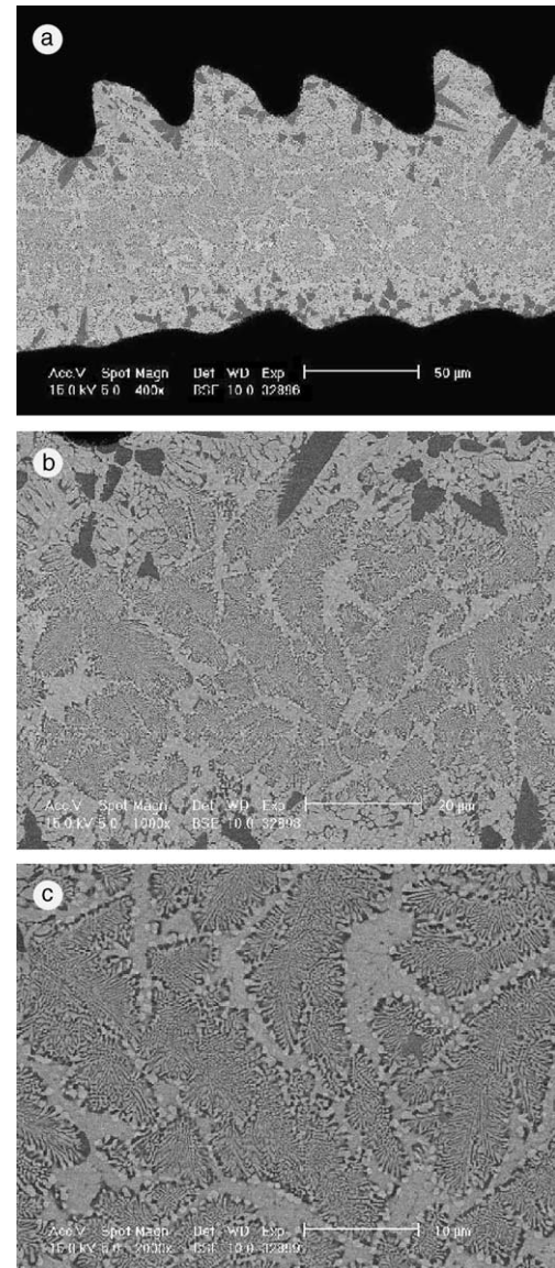
Fig. 5. SEM micrograph of a cross-section of a chip cut at 1.52 m/s. (a) 400 \times , (b) 1000 \times , (c) 2000 \times . Contrast is due to back-scattered secondary electrons (BSE).
