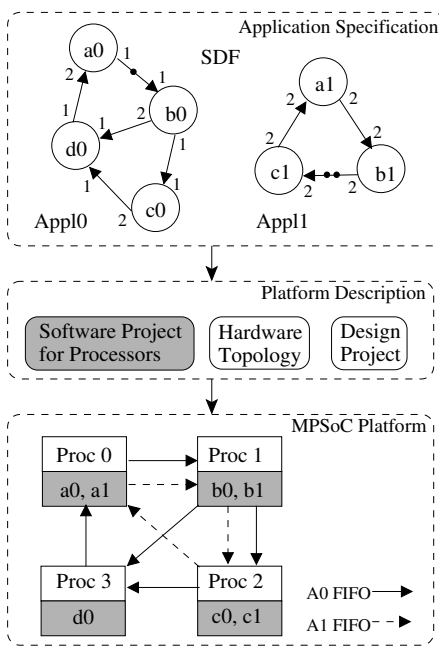
Fig. 3. Design flow
