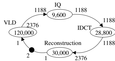
Fig. 5. SDF graph for H263 application
