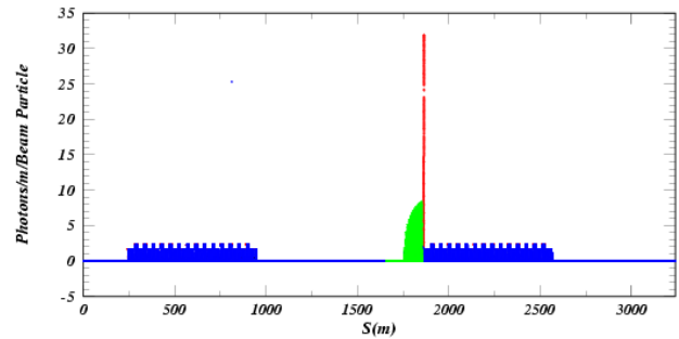
Figure 1: Photon rate ( \gamma/m/\text{beam particle/turn} ) on the outside wall of the vacuum chamber around the DSB3_2 lattice calculated by the Bmad utility SYNRAD. The rates in the field-free regions are shown in blue, those in the dipoles in red, and those in wigglers in green.
