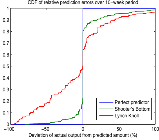
Figure 1: Illustration of the the empirical distribution \mathbf{E}_i constructed from real error data for 3 DERs: 1. A theoretical optimal predictor, 2. A good predictor wind farm (Shooter's Bottom), 3. A poor predictor wind farm (Lynch Knoll)
