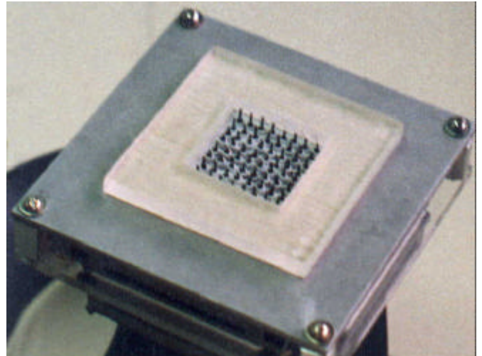
Figure 5. Tactile human interface consisting of an 8-by-8 array of electromagnetic vibrators
