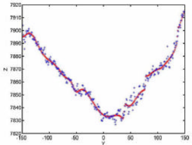
Figure 12. Real and NN modeled ( Y, Z ) geometric profile of a semi-stiff material (cardboard) pressed with a normal force F= 2.65 N. The unit of measurement for both Y and Z axes is 0.1 mm.
