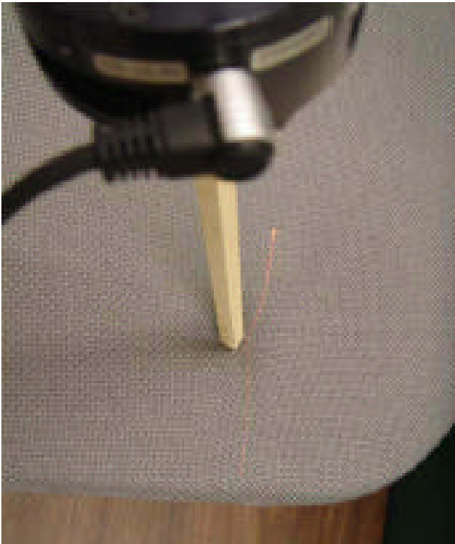
Figure 6. Force-torque sensor measuring the interaction force and torque at the point of contact between the robot manipulated probing rod and the object.
