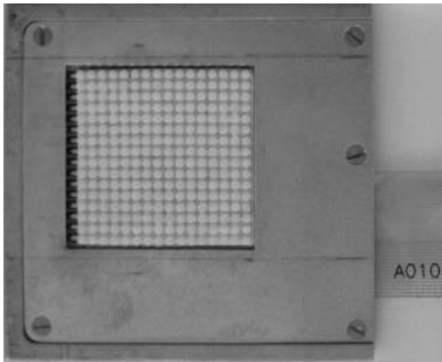
Figure 4. 16-by-16 tactile sensor array.
