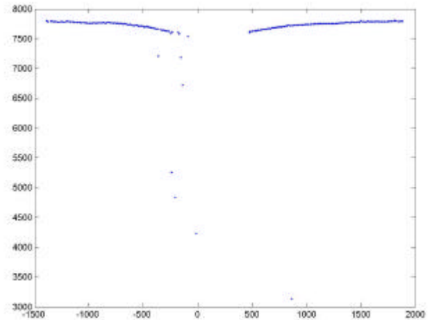
Figure 8. Geometric profile measured by the laser range-finder on the horizontal direction. The unit of measurement for both axes is 0.1 mm.
