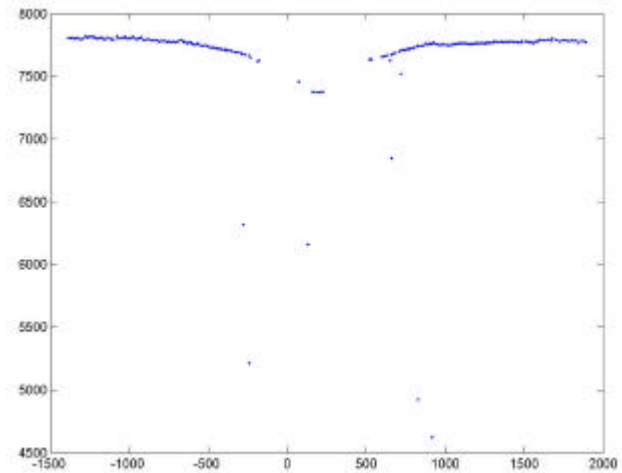
Figure 9. Geometric profile measured by the laser range-finder on the vertical direction. The unit of measurement for both axes is 0.1 mm.
