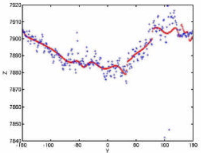
Figure 11. Real and NN modeled ( Y, Z ) geometric profile of a semi-stiff material (cardboard) pressed with a normal force F=0.37 N. The unit of measurement for both Y and Z axes is 0.1 mm.
