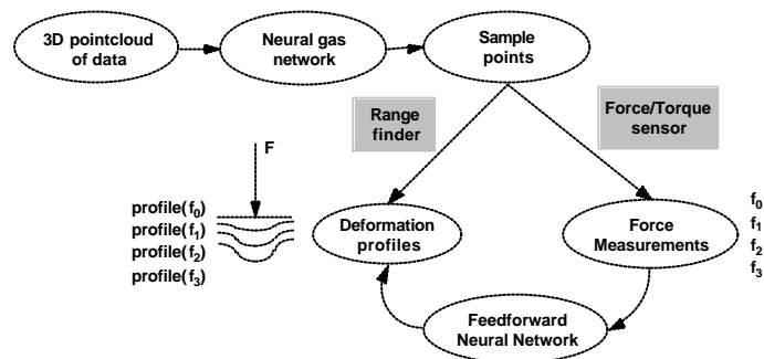
Figure 10. Neural Network mapping and clustering of elastic behavior from tactile and range imaging data.
