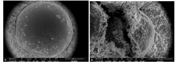
Figure 4: SEM image of microcapsule introduced in cement specimen.
