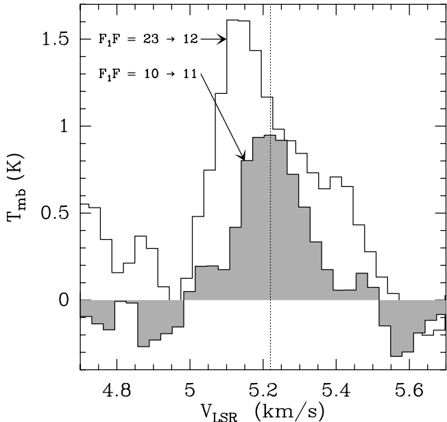
FIG. 3.—Profile of the main F_1, F = 2, 3 \rightarrow 1, 2 hyperfine component of \text{N}_2\text{H}^+(1-0) (open histogram) superposed on the spectrum of the weak F_1, F = 1, 0 \rightarrow 1, 1 component (shaded histogram) at the dust peak position. Note that the weak component is symmetric and peaks where the absorption of the main component is steepest, suggesting that this component is optically thin and can be used to estimate the column density and line width where the main group of hyperfines is affected by self-absorption. [See the electronic edition of the Journal for a color version of this figure.]
