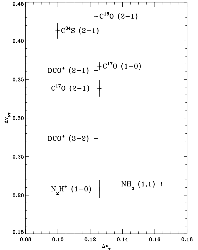
FIG. 6.—Nonthermal line width plotted against the thermal line width for each transition observed, at the position of the dust emission peak. The thermal line width is calculated from an assumed gas temperature of 10 K. The error in the nonthermal line width is derived using the error in the FWHM of the Gaussian fit to the line. The line widths of C^{34}S(2-1) and DCO^+(3-2) are highly uncertain because of the strong absorption observed (see Fig. 2), and the plotted errors do not take the absorption into account. The NH_3 intrinsic line width is taken from Barranco & Goodman (1998). To make a fair comparison, all of the spectral line maps have been spatially smoothed to the \sim 1' resolution of the NH_3 map.
