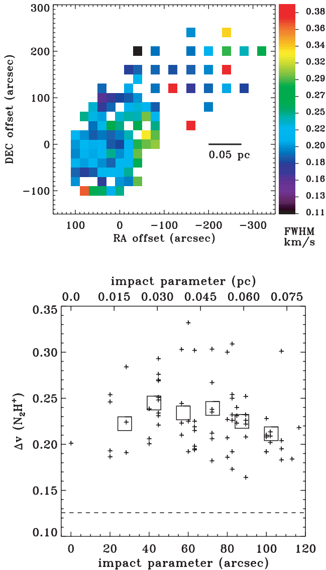
FIG. 5.— Top : N_2H^+(1-0) observed line width across the TMC-1C core. Bottom : N_2H^+(1-0) observed line width (in \text{km s}^{-1} ) vs. distance from the peak of the dust column density map. For those positions where the self-absorption is present, we used the width of the weak component as representative of the intrinsic line width of the (1-0) line. The plus signs show the values at each position in the map with S/N > 3 , and the large squares are averages of the data with 15'' bins. The horizontal dashed line shows the thermal FWHM at 10 K for reference.
