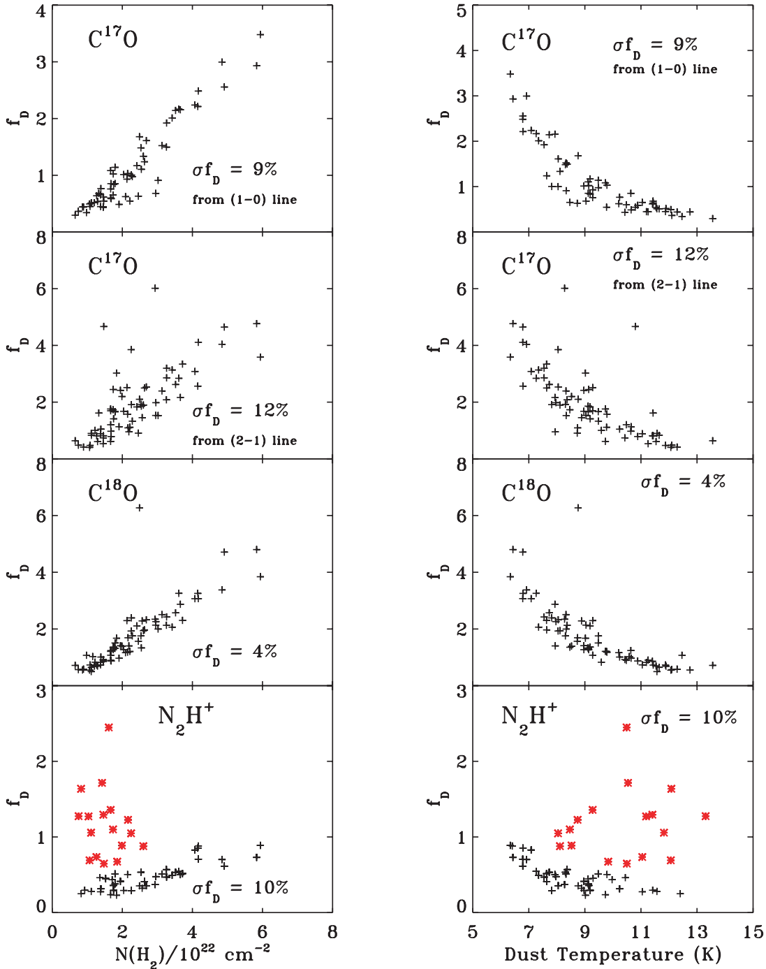
FIG. 14.— Left : Depletion factor derived from molecular transitions observed with the IRAM 30 m plotted against the column density derived from dust emission maps at 450, 850, and 1200 \mu\text{m} . The median percent error in the depletion (calculated from the rms of the spectrum) is given in each panel. Right : Same as left, except that the depletion factor is plotted against the dust temperature. Those points with anomalously high \text{N}_2\text{H}^+ depletion factors ( N_{\text{H}_2} < 3 \times 10^{22} and f_D > 0.6 ) are shown in red, and their positions are shown with plus signs in Fig. 4. The \text{N}_2\text{H}^+ depletion factor goes below 1 because of our arbitrary choice of the \text{N}_2\text{H}^+ column density (see text).
