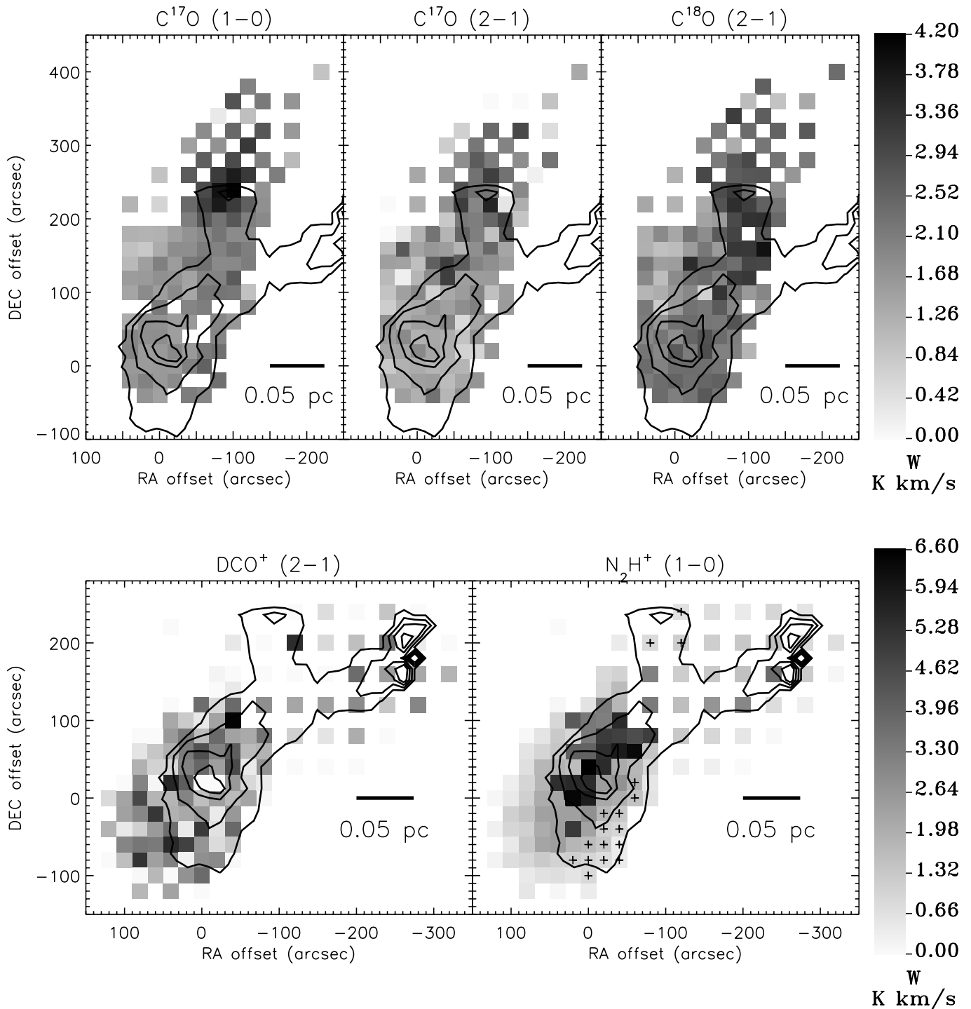
FIG. 4.—Integrated intensity maps of C^{17}O(1-0) (top left), C^{17}O(2-1) (top middle), C^{18}O(2-1) (top right), DCO^+(2-1) (bottom left), and N_2H^+(1-0) (bottom right). The C^{17}O(1-0) , C^{17}O(2-1) , and DCO^+(2-1) integrated intensities have been scaled up by factors of 1.5, 2.0, and 5.0, respectively. For all spectra showing self-absorption, the N_2H^+ integrated intensity has been calculated from the thinnest hyperfine component. The contours show the visual extinction derived from the dust emission, at levels of A_V = 10, 25, 40, and 55 mag. The 1\sigma uncertainties in the integrated intensity are \sim 0.05, \sim 0.06, \sim 0.10, \sim 0.07, and \sim 0.08 K km s ^{-1} in C^{17}O(1-0), C^{17}O(2-1), C^{18}O(2-1), DCO^+(2-1), and N_2H^+(1-0) , respectively. The positions with large N_2H^+ depletion and low column density have been marked with plus signs. [See the electronic edition of the Journal for a color version of this figure.]
