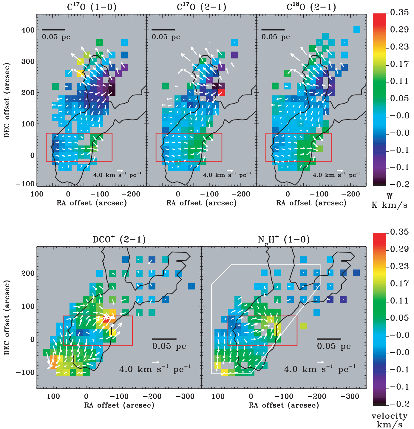
FIG. 7.— Top : Velocity fields for C^{17}O(1-0) , C^{17}O(2-1) , and C^{18}O(2-1) . The black contour shows the A_V = 10 mag boundary, and the arrows show the direction and magnitude of the line-of-sight velocity gradient, pointing from blue to red. The red box encloses a region with a velocity gradient similar to that of rotation seen in the isotopologues of CO. In each map the velocity shown is the difference between the measured velocity relative to LSR (VLSR) at each position and the velocity at the (0, 0) position. The lengths of the arrows are proportional to the magnitude of the gradient, and are scaled to the labeled arrow. Bottom : Velocity fields for DCO^+(2-1) and N_2H^+(1-0) in TMC-1C. The red box encloses a region with a velocity gradient in isotopologues of CO that looks similar to that of rotation. The white box shows the region observed in NH_3 by Barranco & Goodman (1998).
