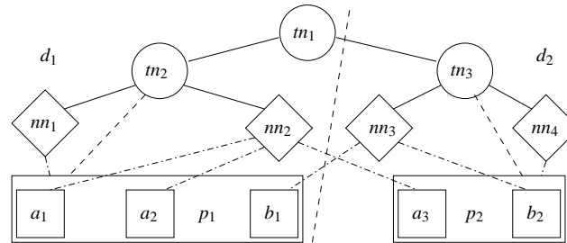
Figure 3: A decomposition tree. Square nodes denote packs while negotiation nodes have a diamond shape. The remaining tree nodes are depicted circular. The packs and the nodes are hosted by two devices d_1 and d_2 , separated by the dotted border.
