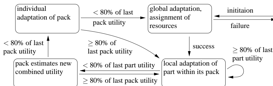
Figure 2: Life cycle of a resource negotiation node. Note that only the regular state transitions are shown. The figure does not show transitions taken in exceptional situations, e.g. , when new packs are established and when large amounts of free resources become available. Transitions labeled with “80%” refer to estimates compared to the last calculated utility.
