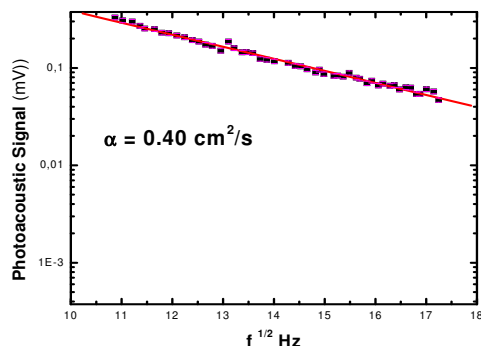
Fig. 11. Thermal diffusivity of the 5 GPa/1400°C/2 min HPHT sintered hardmetal
