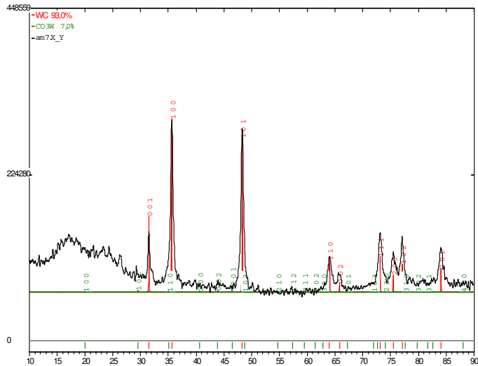
Fig. 10. Rietveld Analysis for the 5 GPa/1200°C/1min sample
