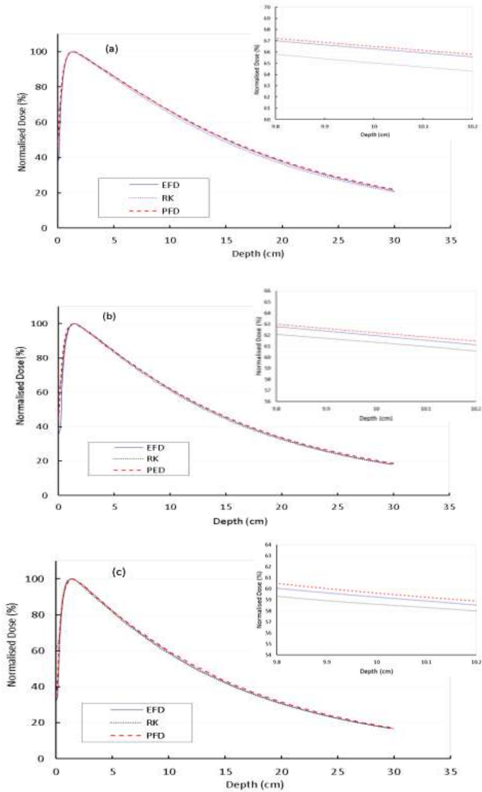
Figure 1. Percentage depth dose curves for different field sizes: a) 10 \times 10 \text{ cm}^2 , b) 5 \times 5 \text{ cm}^2 , and c) 3 \times 3 \text{ cm}^2 (EFD: electron field detector, PFD: photon field detector, RK: RK ionization chamber).
