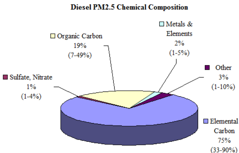
Figure 4. Typical chemical compositions for diesel particulate matter (PM 2.5 ) (EPA, 2002a)
