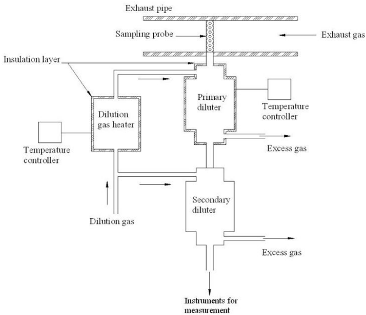
Figure 1. Schematic of a typical dilution tunnel.
