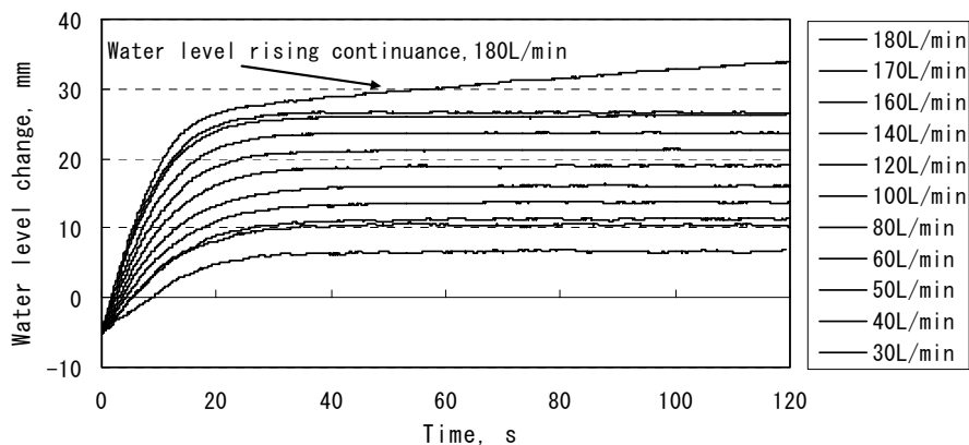
Figure 5 Flow rate and water level change in V500
