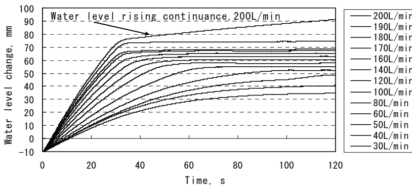
Figure 7 Flow rate and water level change in H500
