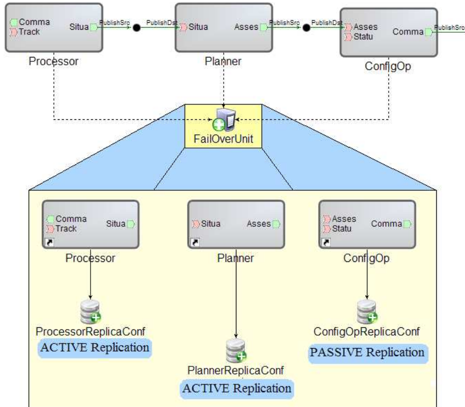
Figure 3: Availability Requirements Modeling in CQML
