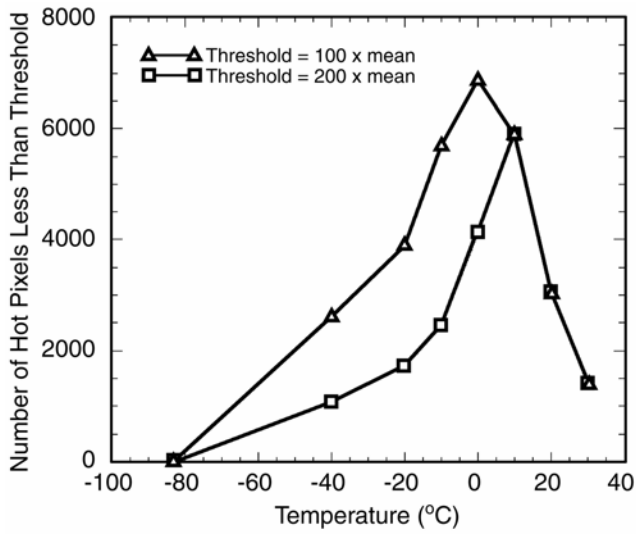
Figure 6. Number of annealed hot pixels versus temperature.
