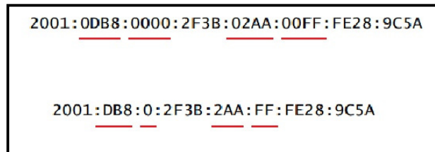
Figure 2. IPv6 addressing
