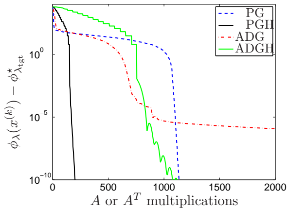
(f) Number of matrix-vector multiplications.
