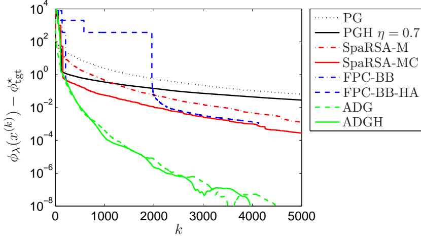
Figure 5: Comparison of different methods for solving a non-sparse random instance.
