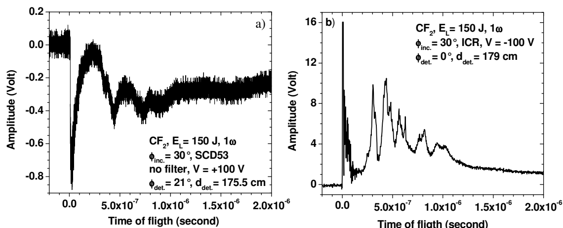
Fig. 3: Typical TOF spectra for diamond (a) and ion collector (b) from PALS experiment.
