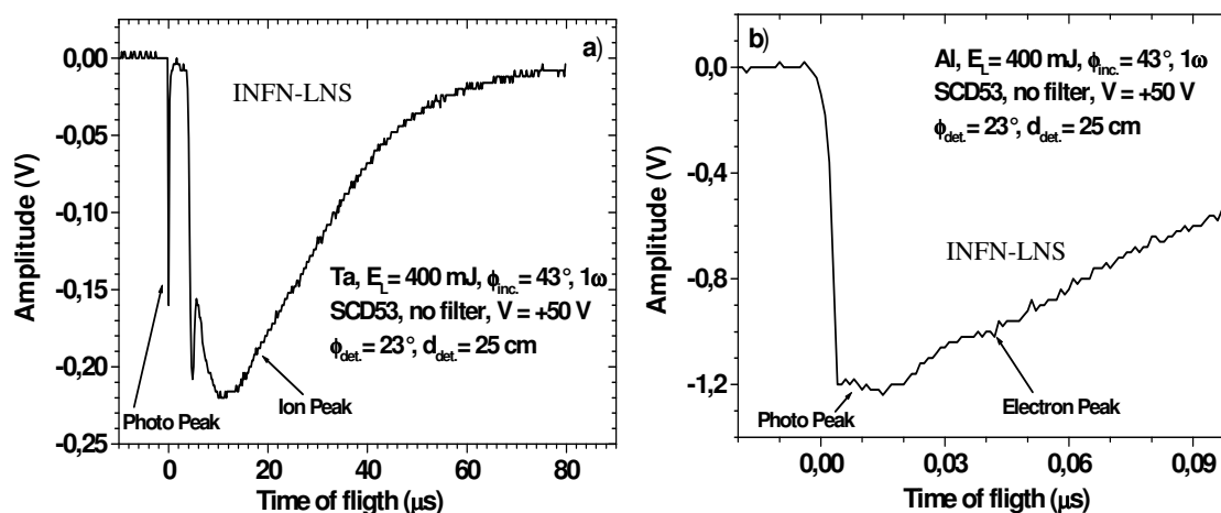
Fig.1: TOF diamond spectra for Ta (a) and Al (b) plasmas obtained at INFN-LNS.
