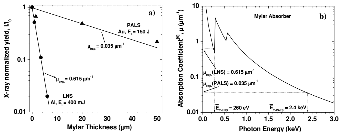
Fig. 2: X-ray yield vs. absorber thickness (a) and absorption coefficient vs. energy (b).
