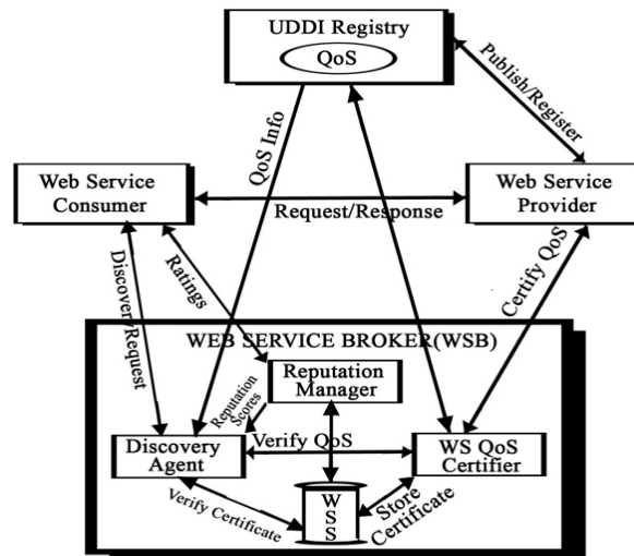
Fig.1: Framework for Agent-based Web Services Discovery with QoS
