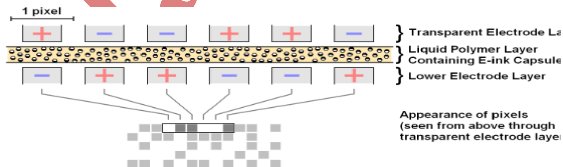
Fig-1: Appearance of pixels seen from transparent electrode layer
