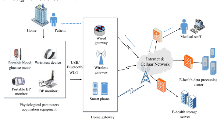
Fig.1. Architecture of CVDs monitoring system
