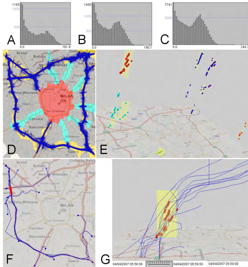
Figure 9.6 A,B,C: Frequency distributions of car speeds on motorways in different ranges of distance to the nearest neighbour car: below 20m (A), 20-50m (B), over 50m (C). D: Trajectory segments on or near motorways selected by means of segment filter. E: Spatio-temporal clusters of low speed events on motorways where the distance to the nearest neighbour is 10m or less. Yellow shapes represent spatio-temporal convex hulls of the clusters. F: Trajectories that passed through one of the convex hulls are selected by filtering. G: The selected trajectories and respective low speed events in a STC.
