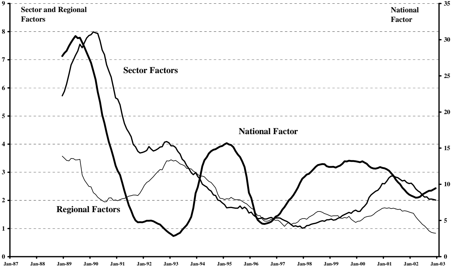
Figure 1: Moving Average National, Sector and Regional MADs
