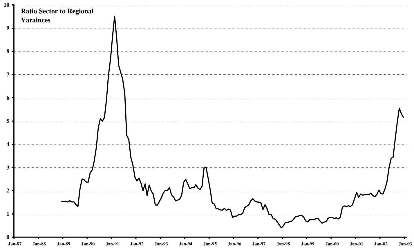
Figure 4: The Ratio of Sector to Regional Variances
