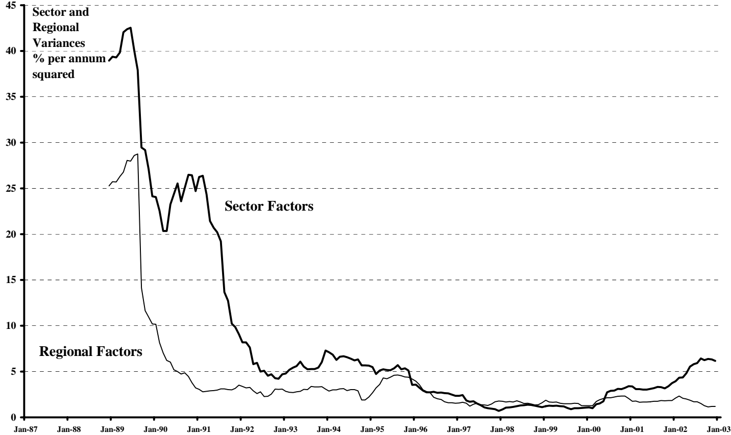
Figure 3: Moving Averages of Sector and Regional Variances
