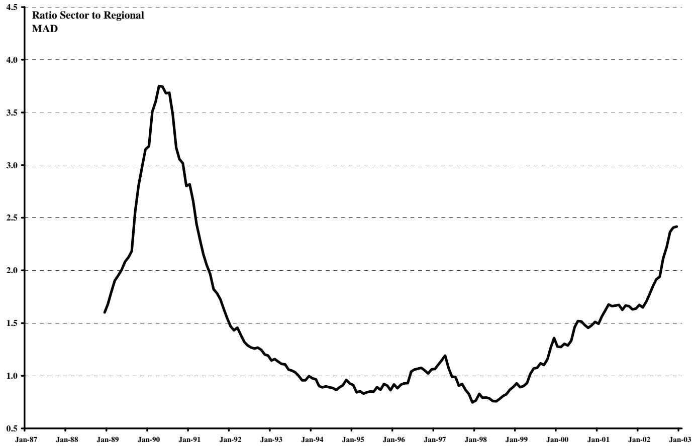
Figure 2: The Ratio of Sector to Regional MADs
