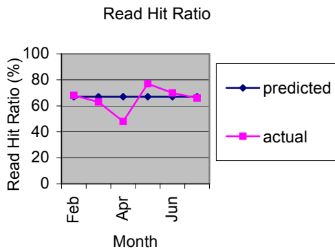
Figure 5. Actual and Predicted Hit Ratio
