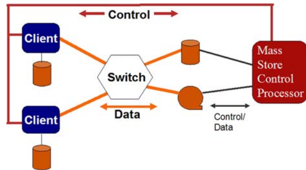
Figure 2. Logical Diagram of NCAR MSS
