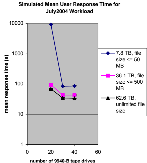
Figure 6. Estimated Response Time for July 2004 Workload
