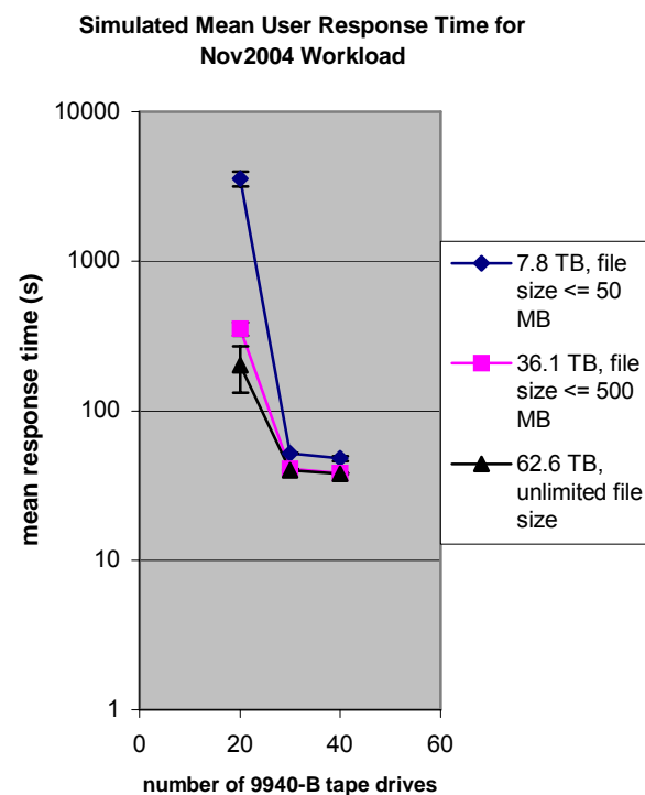
Figure 7. Estimated Response Time for Nov. 2004 Workload
