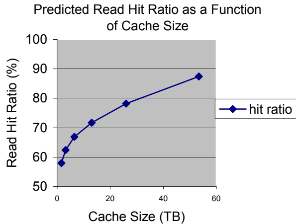
Figure 4. Predicted Hit Ratio
