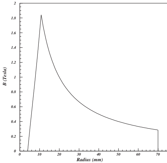
Fig. 6. Magnetic field in the horn as a function of its radius, at the downstream end (the neck) of the horn. The radial position of the inner conductor is between 4 mm and 10.8 mm.
