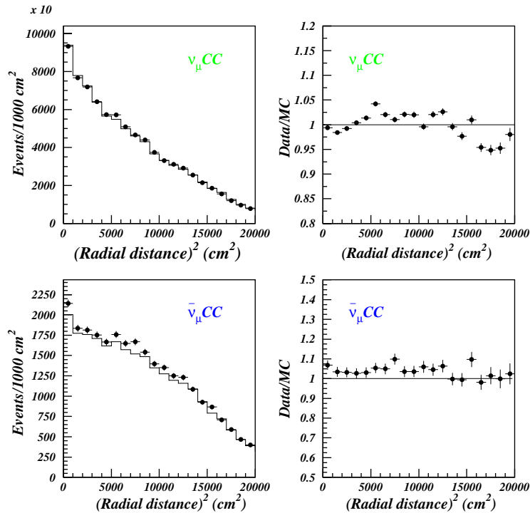
Fig. 19. Left: distributions of the square of the radial position of neutrino interaction vertex for the data (points with error bars) and the Monte Carlo (histogram), for \nu_{\mu}CC (top) and \bar{\nu}_{\mu}CC (bottom) interactions in neutrino mode. Right: ratios of the measured to the predicted distributions. The errors shown are statistical only.
