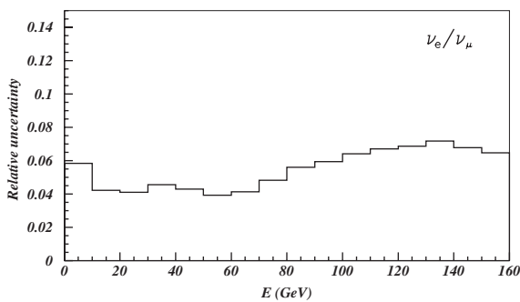
Fig. 15. Total energy-dependent uncertainty on the \nu_e/\nu_\mu ratio. The energy-independent uncertainty is given in Table 5.
