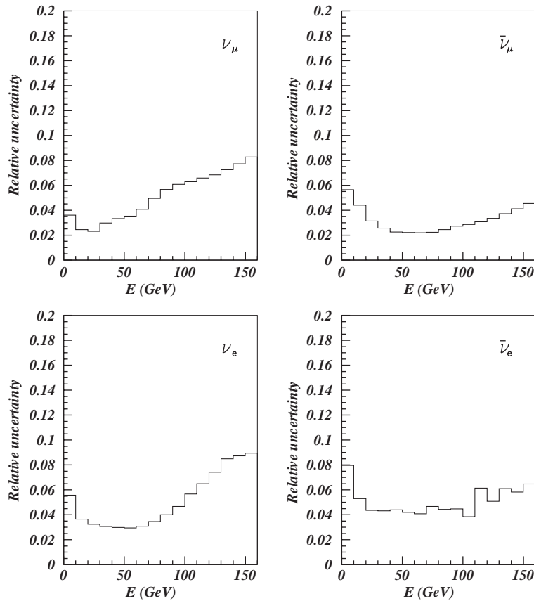
Fig. 14. Total energy-dependent uncertainties on the yields of each of the four neutrino species. The energy-independent uncertainties are listed in Table 5.
