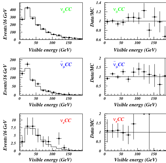
Fig. 18. Left: neutrino energy spectra for the data (points with error bars) and the Monte Carlo (histogram), for \nu_\mu CC (top), \bar{\nu}_\mu CC (middle) and \nu_e CC (bottom) interactions in zero-focusing mode . Right: ratios of the measured to the predicted distributions, for the same three neutrino species. The errors shown are statistical only.
