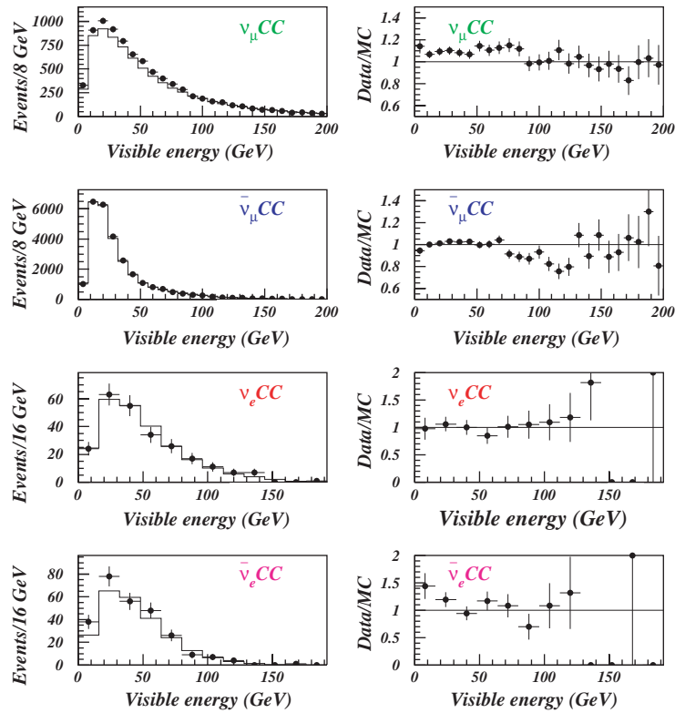
Fig. 17. Left: neutrino energy spectra for the data (points with error bars) and the Monte Carlo (histogram), for (from top to bottom) \nu_\mu CC , \bar{\nu}_\mu CC , \nu_e CC and \bar{\nu}_e CC interactions in antineutrino mode . Right: ratios of the measured to the predicted distributions, for the same four neutrino species. The errors shown are statistical only.
