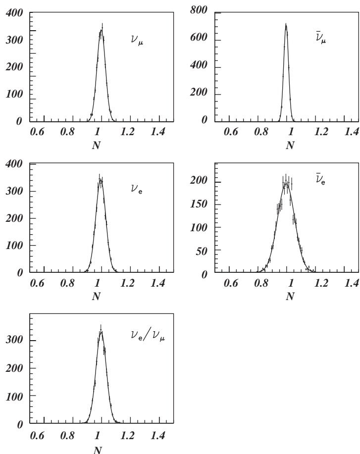
Fig. 13. Distributions of N for each of the four neutrino species and for the \nu_e/\nu_\mu ratio.
