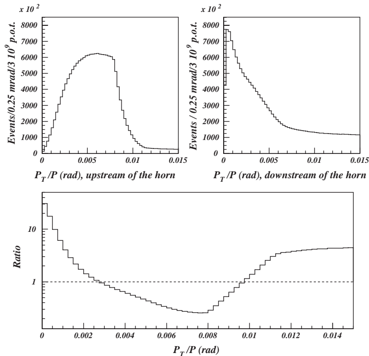
Fig. 7. Distribution of the angle between the \pi^+ momentum vector and the beam line direction, p_T/p , just upstream of the horn (top left), right after it (top right) and the ratio of the latter to the former (bottom).
