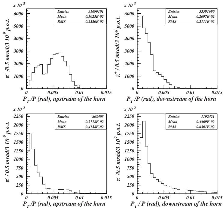
Fig. 9. Distribution of the angle between the pion momentum vector and the beam line direction, p_T/p , just upstream of the horn (left) and immediately after it (right), for \pi^+ producing a \nu_\mu at NOMAD (top) and \pi^- producing a \bar{\nu}_\mu (bottom).
