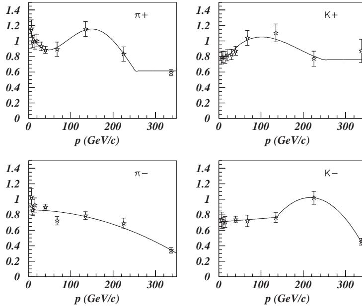
Fig. 5. The reweighting functions for \pi^+ , K^+ , \pi^- and K^- obtained from the SPY and NA20 measurements. The points are the weights calculated for the values of p for which the measurements were made, the curves are the result of fitting them with combinations of polynomial functions.
