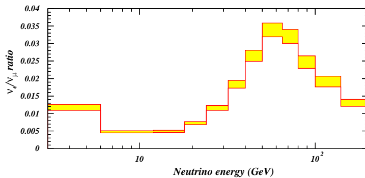
Fig. 20. Ratio \nu_e/\nu_{\mu} as a function of neutrino energy at NOMAD, within the transverse fiducial area of 260 \times 260 cm 2 . The upper and lower boundaries of the filled band correspond to the predictions with \pm 1\sigma uncertainty, where \sigma includes both the normalization and energy-dependent uncertainties added in quadrature.
