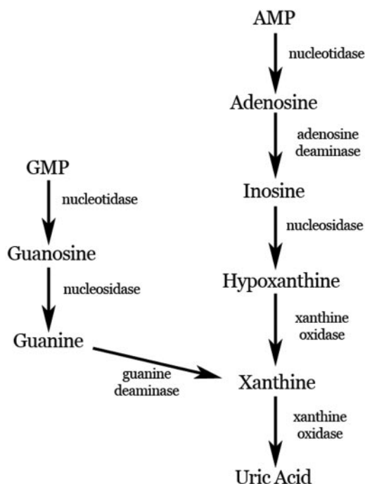
Fig. 1. Purine metabolism leads to the production of uric acid.
