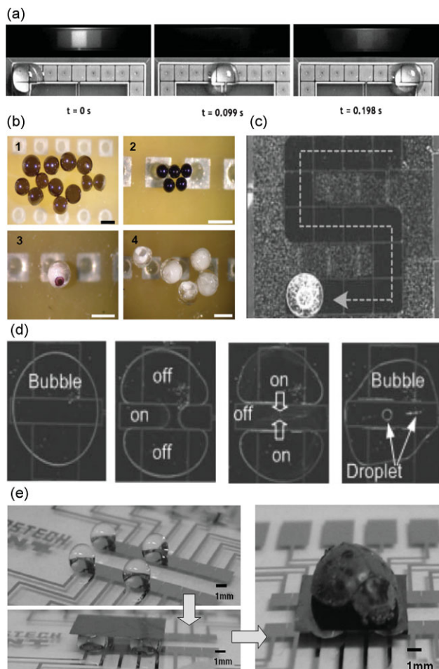
Figure 3. Nonbiological applications of DMF. a) Pictures depicting the use of DMF to cool an artificial hot spot (an imbedded microheater). The top half of each frame shows an infrared image of the hot spot (white = hot); the temperature drops significantly during and after the droplet passes over it. Reproduced with permission from [19]. Copyright 2008 IEEE. b) Pictures depicting particles being synthesized using DMF. The products include conductive gold/SU-8 particles (1), semiconducting polypyrrole particles (2), “eyeball” microbeads (3), and “cups”, formed by drying water droplets that were originally encapsulated in latex (4). Scale bars: 1 mm. Reprinted with permission from [40]. Copyright 2005 Nature Publishing Group. c) Figure depicting a droplet sampling particles on the surface of a DMF device. Reproduced with permission from [42]. Copyright 2006 The Royal Society of Chemistry. d) Frames from a movie depicting bubble splitting and merging on a DMF device. Reproduced with permission from [44]. Copyright 2007 The Royal Society of Chemistry. e) Pictures of a microbelt conveyer system based on DMF; the picture on the right shows a lady bug carried on a silicon wafer supported by four droplets. Reproduced with permission from [45]. Copyright 2006 Elsevier B.V.
