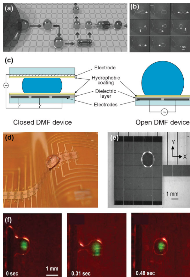
Figure 1. The DMF paradigm. a) Schematic and b) pictures from a movie depicting the four principle DMF processes: dispensing, moving, splitting, and merging. Reproduced with permission from [5,7]. Copyright 2006, 2007 IEEE, respectively. c) Schematics of closed and open DMF devices. d) Picture of an ATDA device, capable of manipulating droplets on flexible substrates. Reproduced with permission from [11]. Copyright 2008 The Royal Society of Chemistry. e) Picture of a DMF device powered by a cross-reference electrode array. Reproduced with permission from [17]. Copyright 2003 IEEE. f) Series of pictures from a video (left-to-right) depicting droplet dispensing on an optically driven DMF device. Reproduced with permission from [20]. Copyright 2008 IEEE.
