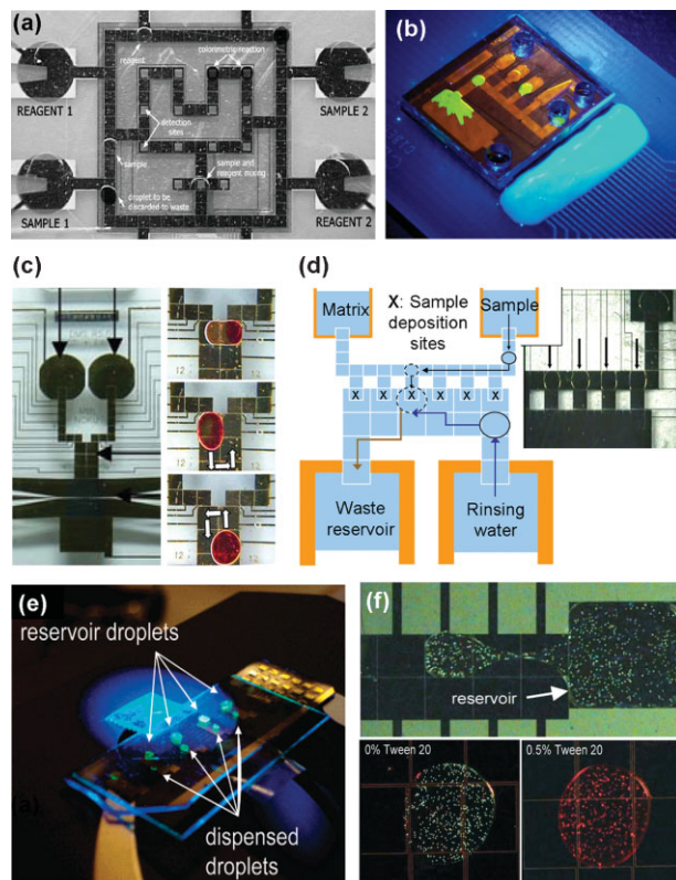
Figure 2. Biological applications of DMF. a) Picture of DMF device used to perform glucose assays. Reproduced with permission from [10]. Copyright 2004 The Royal Society of Chemistry. b) Picture of DMF device used to implement DNA repair reactions. Reproduced with permission from [27]. Copyright 2006 NanoScience and Technology Institute. c) Picture of DMF device used to perform PCR; the pictures on the right are frames from a video depicting the mixing of target DNA and reagents/primers, by moving a merged droplet in circles. Reproduced with permission from [29]. Copyright 2006 Springer Netherlands. d) Schematic and frame from a movie of a DMF device used to perform multiplexed proteomic sample preparation. Reproduced with permission from [12]. Copyright 2006 The Royal Society of Chemistry. e) Picture of a multiplexed DMF device used to study enzyme kinetics. Reproduced with permission from [34]. Copyright 2008 The American Chemical Society. f) Pictures of DMF device used for cell-based toxicity assays. The main panel depicts the dispensing of a droplet carrying Jurkat-T cells labeled with calcein AM (which fluoresces green). The two frames below depict droplets containing cells challenged with 0% (left) and 0.5% (right) Tween 20. Cells exposed to high concentrations of Tween 20 die and fluoresce red when labeled with ethidium homodimer-1. Reproduced with permission from [35]. Copyright 2008 The Royal Society of Chemistry.
