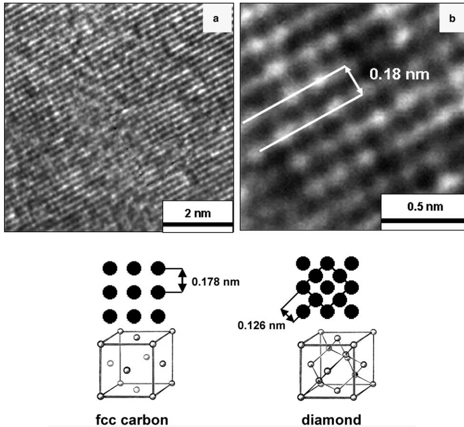
Fig. 9. HRTEM image of the (100) crystal plane of fcc carbon: (a) and (b) the same region of the film at different magnifications; schematic drawings illustrating the crystal lattice of fcc carbon and diamond.
