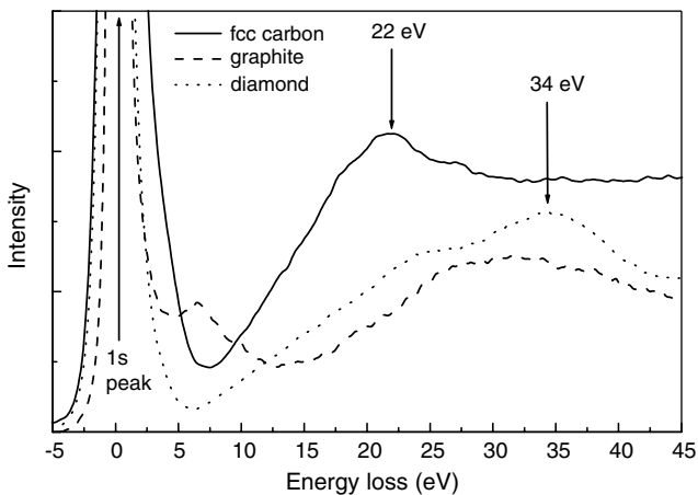
Fig. 8. Electron-energy loss spectrum from fcc carbon compared to that from different carbon allotropes.
