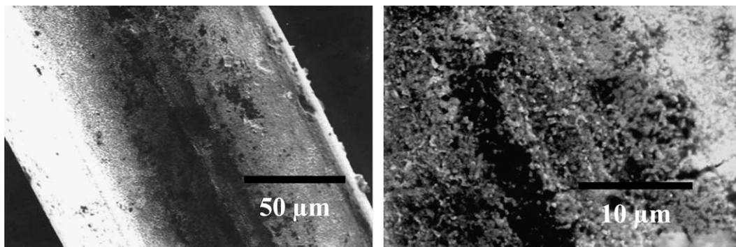
Fig. 2. Surface morphology of a film of fcc carbon deposited on a Ni-wire by HFCVD.
