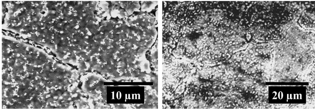
Fig. 3. Surface morphology of a film of fcc carbon deposited on a Ni-sheet by PACVD.
