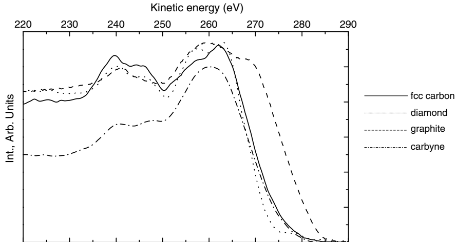
Fig. 6. Carbon peak in the Auger spectra from fcc carbon compared to that from different carbon allotropes.
