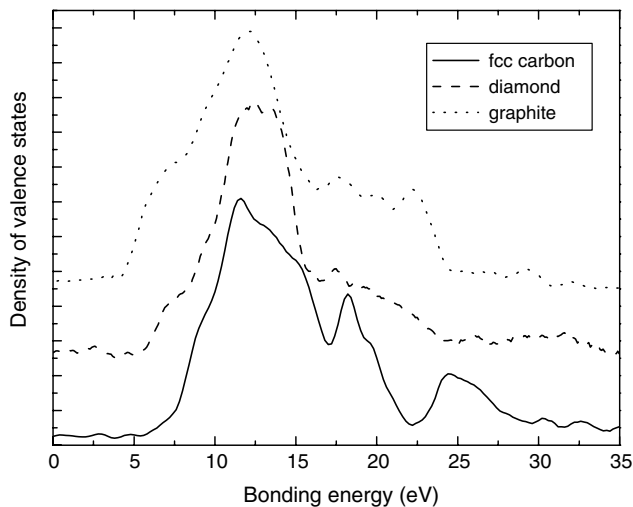
Fig. 7. Density of electron states in fcc carbon compared to that in different carbon allotropes.
