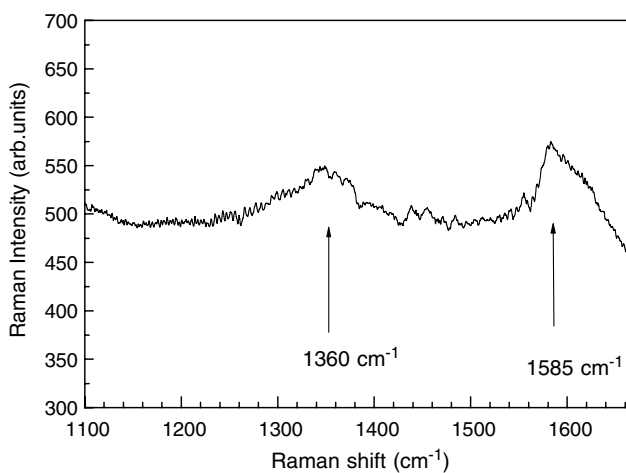
Fig. 5. Raman spectrum from fcc carbon.
