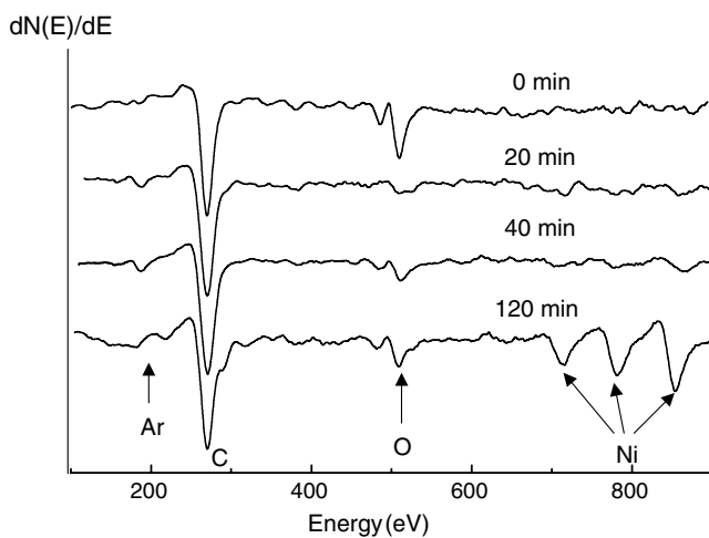
Fig. 4. Auger spectra from the film of fcc carbon deposited by PACVD after various time of Ar etching.
