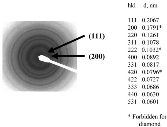
Fig. 1. Electron diffraction from fcc carbon.
