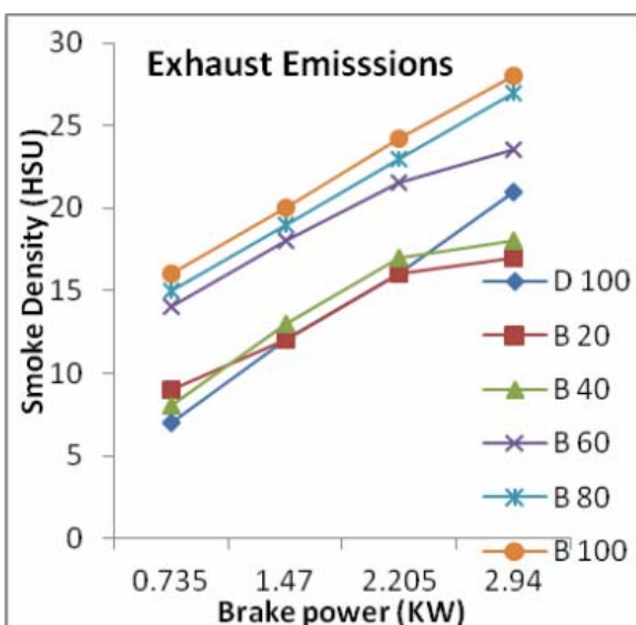
Figure -7. Exhaust emissions. Vs brake power.
