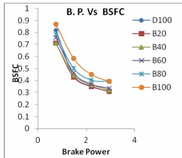
Figure -4. Fuel consumption Vs break power.
