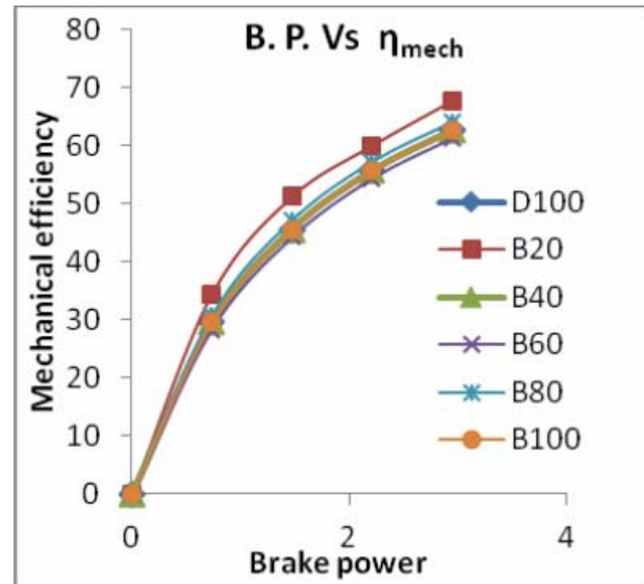
Figure -3. B.P. Vs \eta_{mech} .
