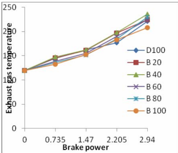
Figure -5. Exhaust gas temp. Vs brake power.
