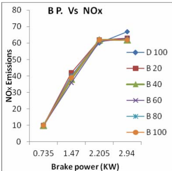
Figure -6. NO x Vs brake power.
