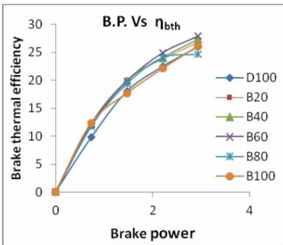
Figure -2. B. P. Vs \eta_{bth} .
