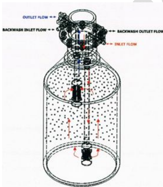
Figure 5a: Filtration mode.
