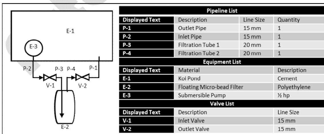
Figure 3: Operation layout of the re-circulating aquaculture system using floating micro-bead bio-filter.
