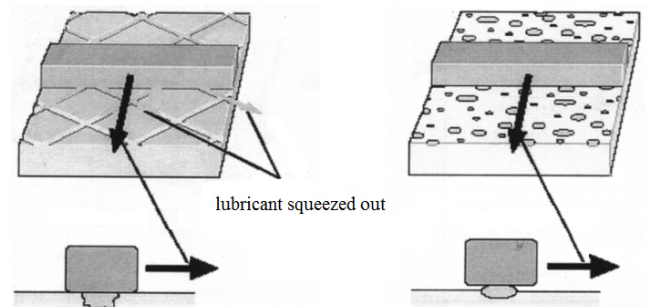
Fig. 1. Schematic diagram showing interaction between grooves and cavities filled with a lubricant on the piston ring/cylinder liner surface contact
