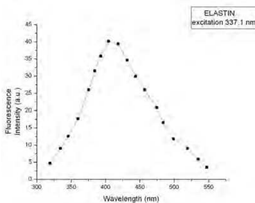
Fig. 9. Fluorescence emitted by elastin excited at 337.1 nm
