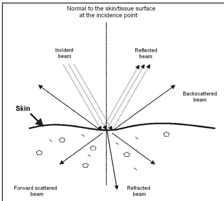
Fig. 13. Laser beam-tissue coupling processes
