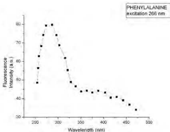
Fig. 3. The phenylalanine fluorescence emission spectrum
