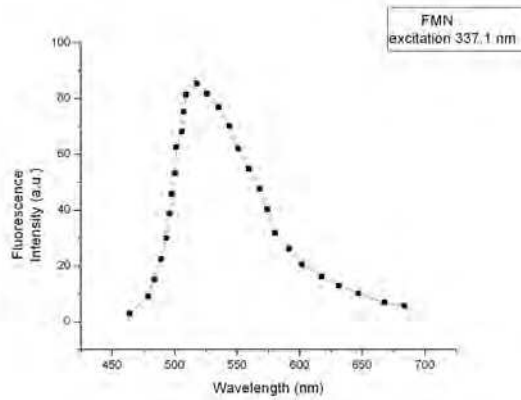
Fig. 10. Fluorescence emitted by FMN
