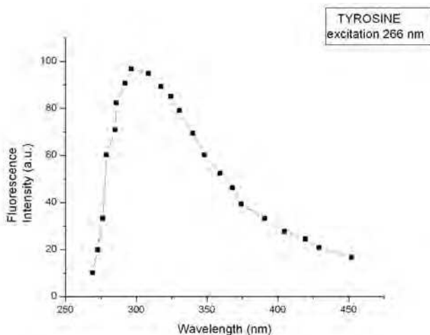
Fig. 5. The tyrosine fluorescence emission spectrum
