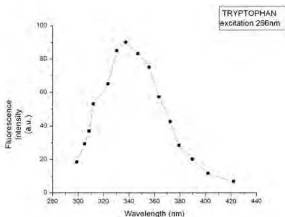
Fig. 4. The tryptophan fluorescence emission spectrum.
