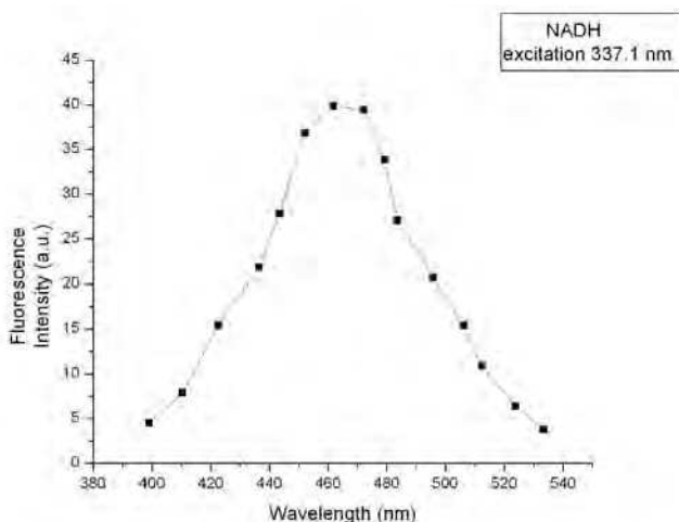
Fig. 6. Fluorescence emission of NADH
