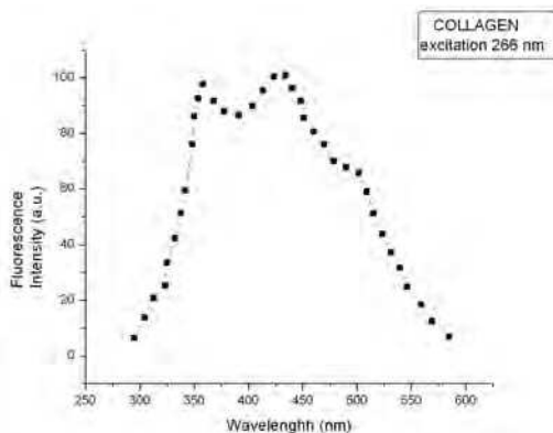
Fig. 7. Fluorescence emitted by collagen excited at 266 nm
