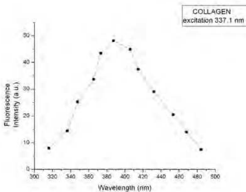
Fig. 8. Fluorescence emission by collagen excited at 337.1nm
