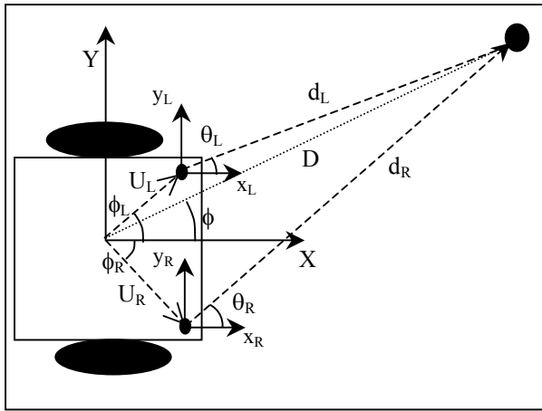
Figure 9. Obstacle detection.
