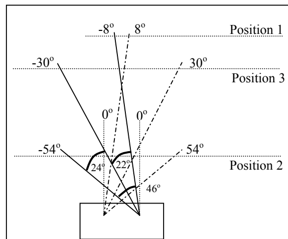
Figure 8. Obstacle detection.
