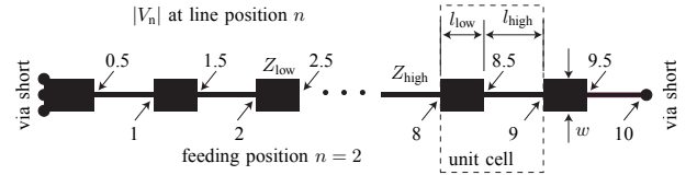
Fig. 10. Microstrip antenna layout: 10 cascaded unit cells with via shorts at the array's ends and voltage monitoring from metalization to ground at the line positions n \in \{0, 0.5, 1, 1.5, 2, 2.5, \dots, 10\} .
