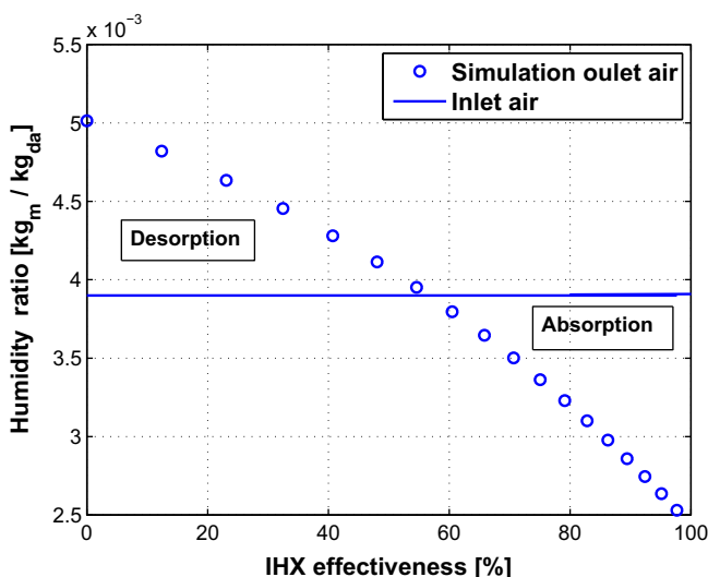
Fig. 6. Outlet humidity ratio versus IHX effectiveness. The continuous horizontal line represent the inlet humidity ratio and circles represent outlet humidity ratio.
