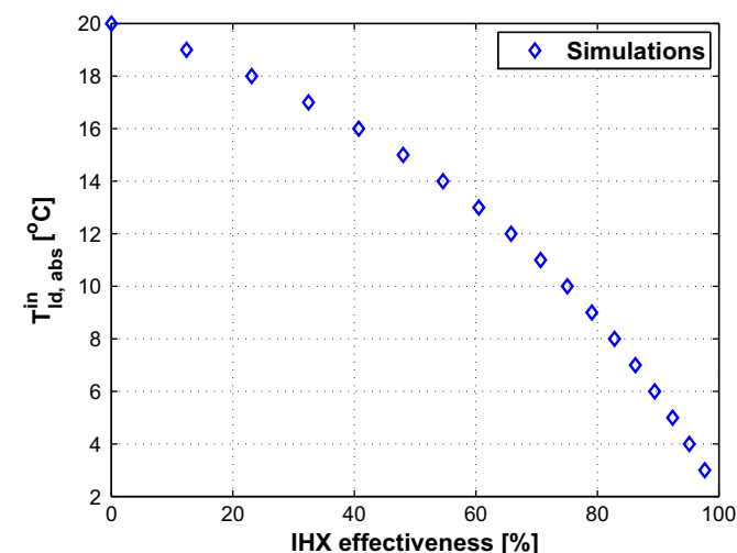
Fig. 4. Inlet liquid desiccant temperature at the absorber as a function of IHX effectiveness. Absorber inlet conditions are: T_a^{\text{in}} = 2^\circ\text{C} , \text{RH}_a^{\text{in}} = 90\% and C_{\text{ld}}^{\text{in}} = 35\% .
