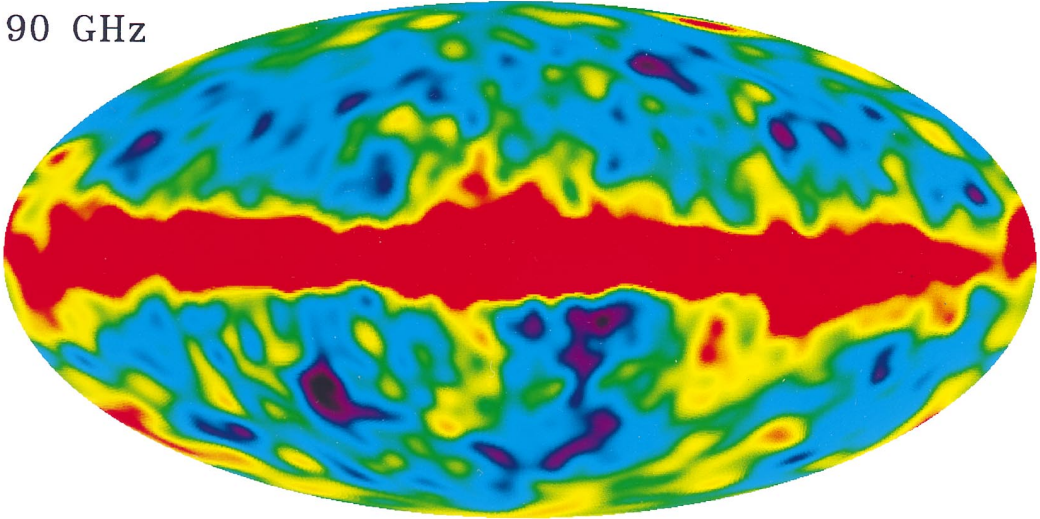
FIG. 1.—Full-sky Mollweide projections of the 31, 53, and 90 GHz 4 yr maps formed by averaging the A and B channels at each frequency. After the mean offset and the dipole are removed, the bright (red) emission from the Galaxy dominates the central band of the maps.
