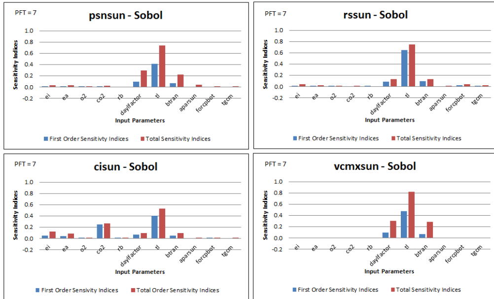
Figure 9. The Sobol Method
