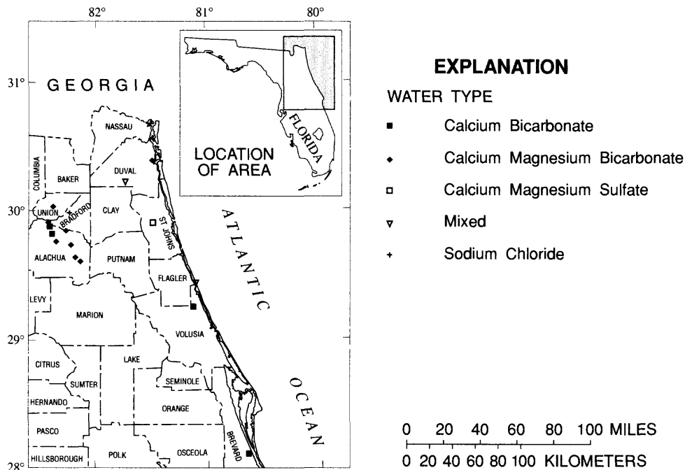
Figure 5. Locations of monitoring wells and dominant-ion water types in samples from wells tapping the intermediate aquifer system in northeastern Florida.
