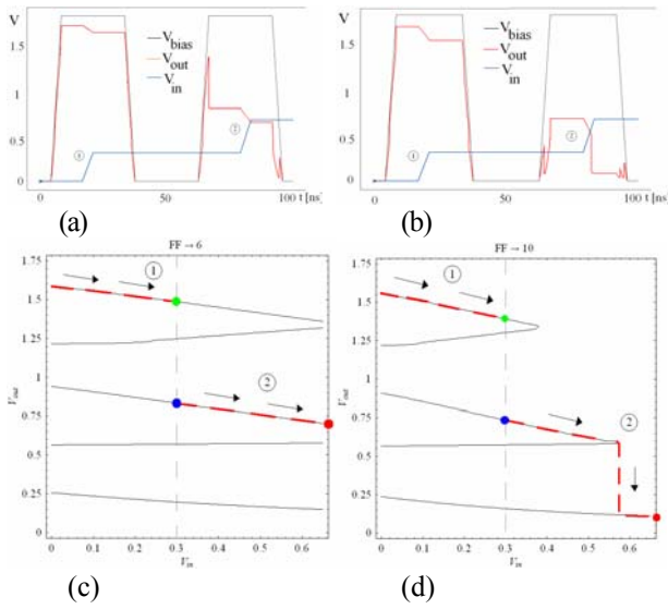
Figure 2. MML ternary inverter with f_z=0.6 , f_y=0.7 , f_B=1.1 and f_A=1.2 . Waveforms for (a) FF=6 (does not exhibit holding problems) and (b) FF=10 (holding disappearance when the input node changes from V_{in}^M to V_{in}^H ). V_{in} - V_{out} plots corresponding to (c) FF=6 and (d) FF=10 .
