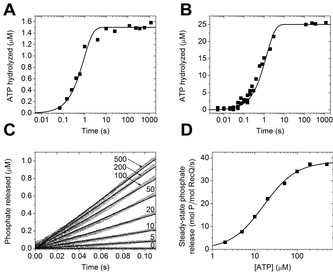
Figure 3. Rate-limiting ATP hydrolysis is markedly accelerated by DNA. Single (A) and multiple (B) turnover quenched-flow time courses of ATP hydrolysis, recorded upon mixing 2- \mu\text{M} RecQ plus 3- \mu\text{M} dT 54 with 1.5- \mu\text{M} (A) or 25- \mu\text{M} (B) \gamma - 32 P-ATP. Lines show global best-fits based on the model of Figure 1A. (C) Stopped-flow time courses of P i release recorded as in Figure 2C but in the presence of 0.5- \mu\text{M} dT 54 (pre-mixed with RecQ). (D) Steady-state ATPase (P i production) activities determined from the slopes of linear fits (lines in (C)). Line shows best-fit using the Hill equation. Determined parameters are listed in Table 1.
