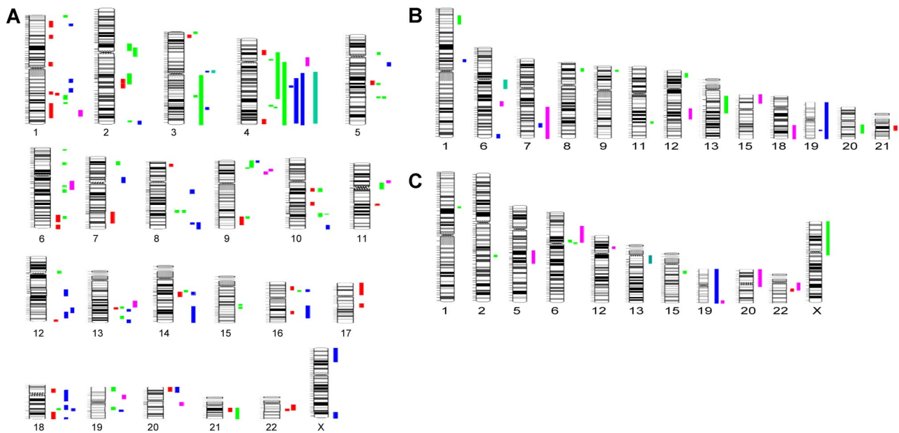
Figure 1. Genomic ideogram showing the distribution of LOH in low-risk MDS patients detected using the 250K SNP assay. Chromosome numbers are below each ideogram. (A) Distribution of UPD greater than 2Mb is shown. One hundred twenty-five regions of UPD were detected: red 5q- Syndrome (n = 33 regions); green RA+RCMDnc (n = 46 regions); blue RARS+RCMD-RS (n = 34 regions); pink RCMDac (n = 10 regions); and green RAEB (n = 2 regions). (B,C) Regions of deletions (del) and amplifications (amp) are shown. CN changes detected: red 5q- syndrome (del, n = 1 region); green RA+RCMDnc (del, n = 7 regions; amp, n = 7 regions); blue RARS+RCMD-RS (del, n = 5 regions; amp, n = 1 region); pink RCMDac (del, n = 5 regions; amp, n = 6 regions); and green RAEB (del, n = 1 region; amp, n = 1 region).
