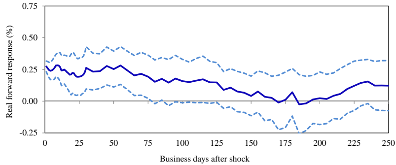
Fig. 4. Impulse response of ten-year US forwards to short-term nominal rates. Panel A plots the coefficient b_{\mathcal{S}}(k) from estimating Eq. (11), using all days from 1987 to February 2012:
