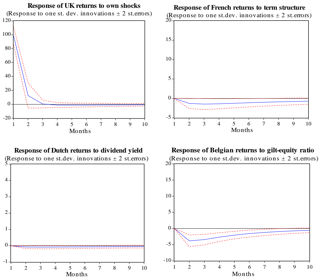
Figure 2: Impulse-Response Functions
