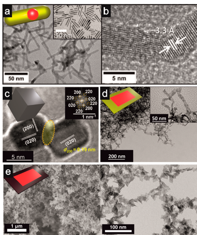
Figure 2. Examples for NC-based gels from shape- and composition-controlled building blocks: (a, b) CdSe/CdS dot/rod NCs, (c) Pt cubes, (d) CdSe/CdS core/crown nanoplatelets (NPLs), and CdSe/CdTe core/crown nanoplatelets as schematically displayed in the top left corner for each material. (a) Gels from CdSe/CdS dot/rod NCs and (inset) the rod building blocks and (b) higher magnification of the connection between the building blocks. Adapted from ref 48. Copyright 2015 Wiley-VCH Verlag GmbH & Co KGaA, Weinheim. (c) High resolution image of interconnected Pt nanocubes forming 3D network with only (100) as the exposed crystal facet. Adapted from ref 44. Copyright 2017 American Chemical Society. (d) TEM micrograph of an aerogel from CdSe/CdS core/crown NPLs. Adapted from ref 41. Copyright 2016 American Chemical Society. (e) (left) SEM and (right) TEM images of aerogel structures obtained from CdSe/CdTe core/crown NPLs. Adapted from ref 1. Published by WILEY-VCH Verlag GmbH & Co. KGaA, Weinheim.
