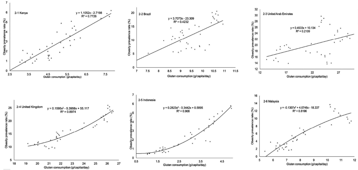
Fig. 2. Country-specific correlation of gluten consumption and obesity in 30 consecutive years (1975–2013) Data sources: Gluten consumption data from the FAO; Obesity prevalence rate from the WHO.
