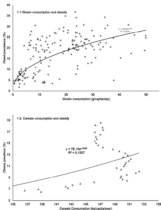
Fig. 1. Worldwide associations between obesity prevalence and gluten consumption and cereals consumption respectively
