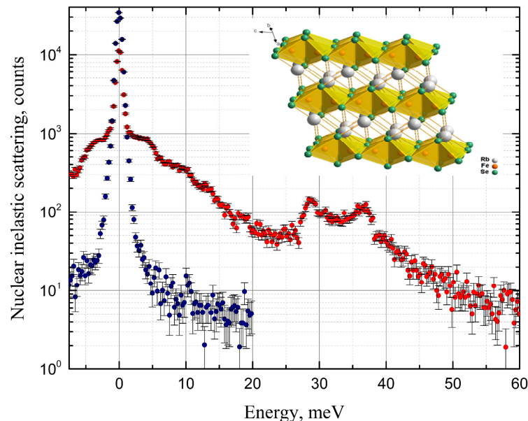
Figure 1. ^{57}\text{Fe} nuclear inelastic scattering spectrum of \text{RbFeSe}_2 (red dots) and instrumental function (blue dots). The inset displays a fragment of the \text{RbFeSe}_2 crystal structure showing quasi-one-dimensional structure of edge-sharing ( \text{FeSe}_4 ) tetrahedra.
