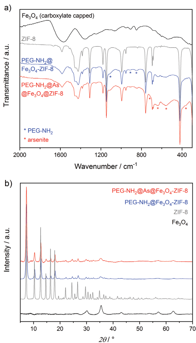
Figure 2. a) FT-IR spectra in the area from 2000 to 300\text{ cm}^{-1} and b) XRPD pattern of \text{Fe}_3\text{O}_4 (black), ZIF-8 (grey), \text{PEG-NH}_2@Fe_3O_4 -ZIF-8 (blue), and \text{PEG-NH}_2@As@Fe_3O_4 -ZIF-8 (red).
