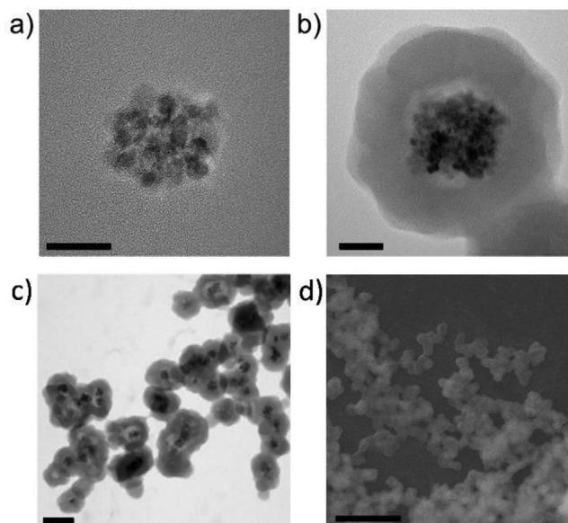
Figure 1. HR TEM micrographs of a) Fe 3 O 4 nanoclusters, b,c) PEG-NH 2 @Fe 3 O 4 -ZIF-8 nanoparticles, and d) a SEM micrograph of PEG-NH 2 @Fe 3 O 4 -ZIF-8 nanoparticles; scale bar: (a,b) 20 nm, (c) 100 nm, (d) 1 μm.
